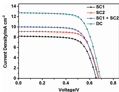
Figure 2. J - V curves of DSSCs sensitized by SC1, SC2, cosensitizers (SC1 + SC2), and DC.
